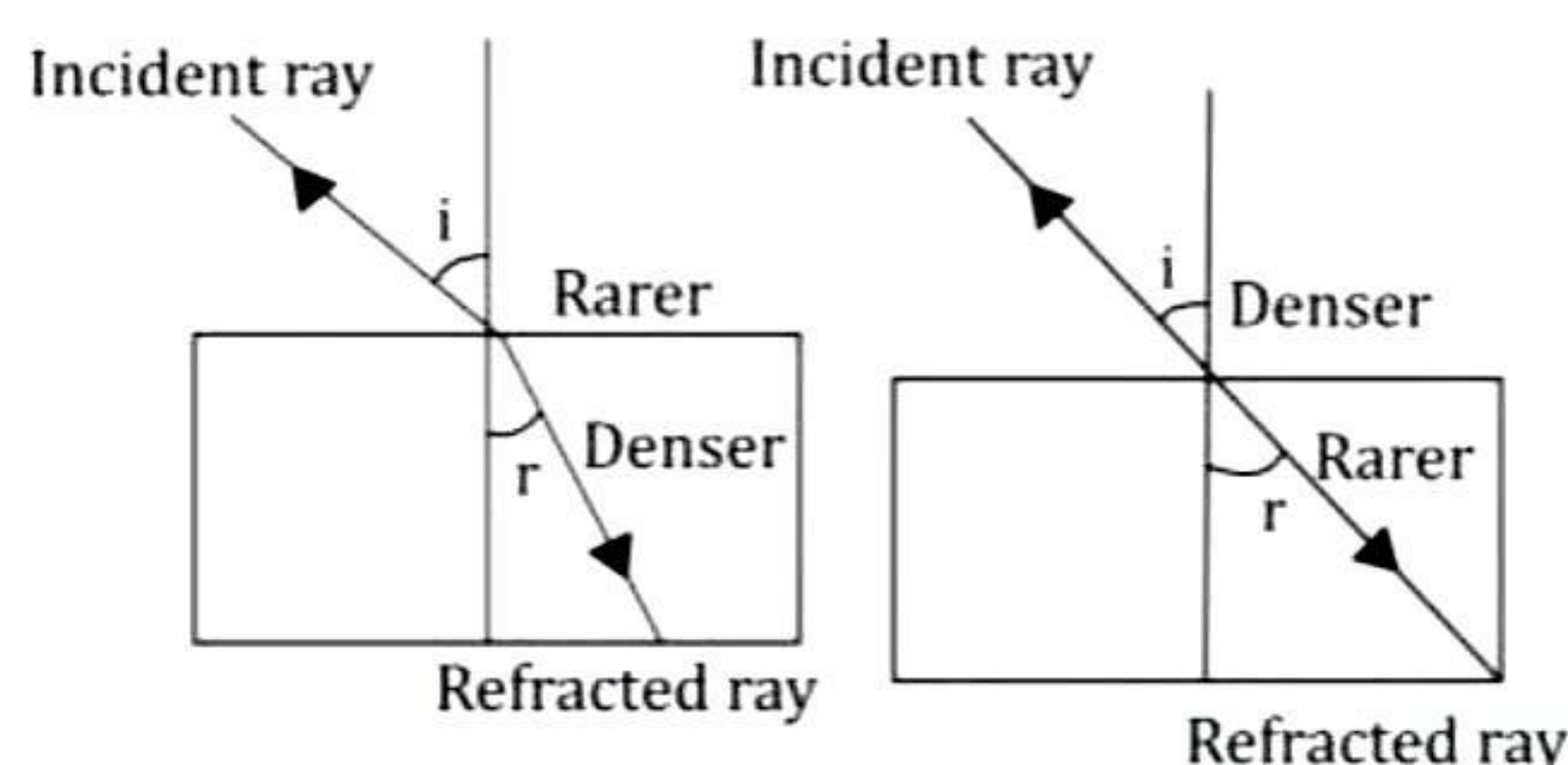
Refraction of light
