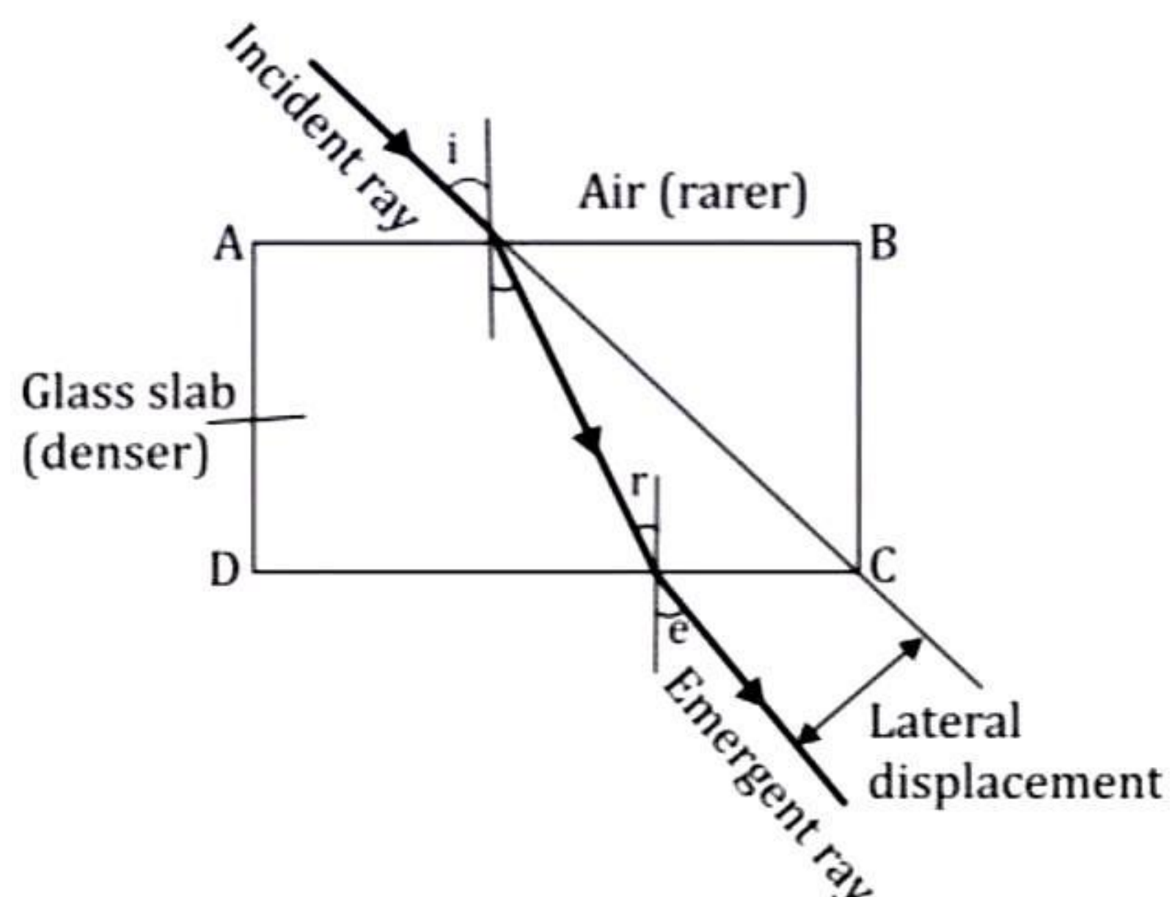
Refraction Through A Rectangular Glass Slab
